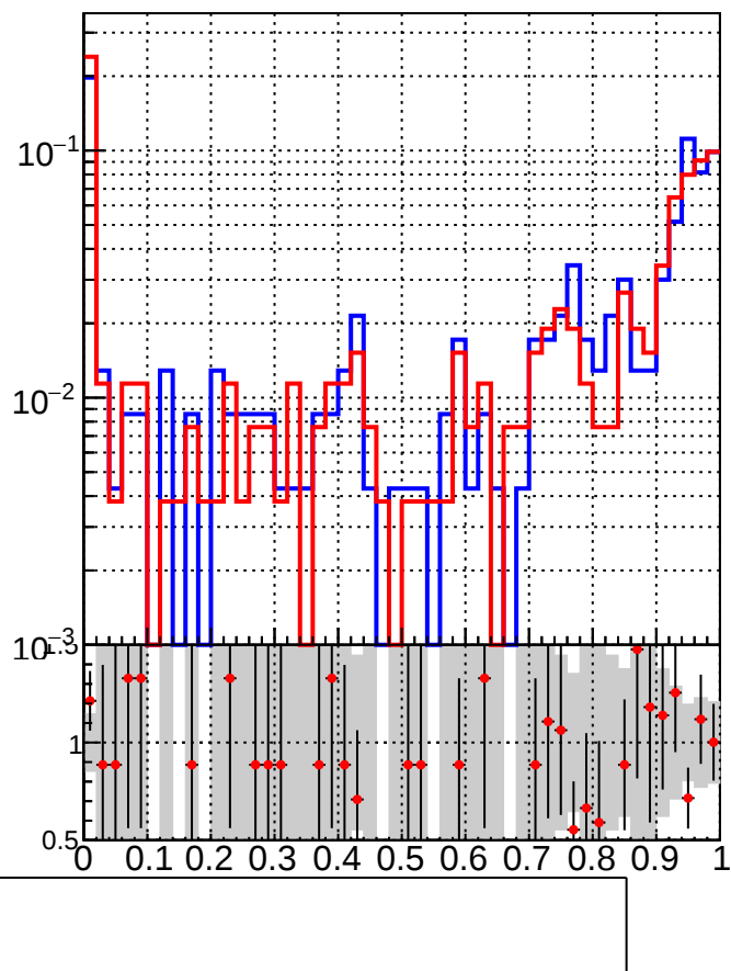
RecoPVAssoc2GenPVNotMatched_missing
