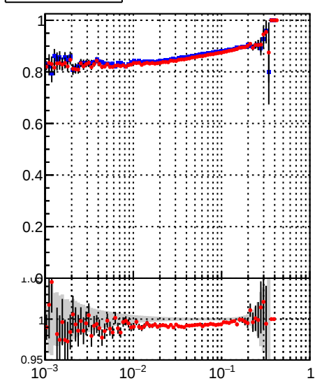
Pileup rate vs \epsilon
