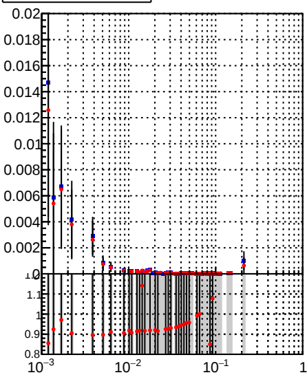
Duplicates Rate vs \epsilon
