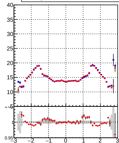
mean hit — DQM_TT_mkFit_ — DQM_TT_mkFit_BDT_
