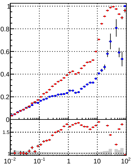
—•— DQM_TT_mkFit_ —•— DQM_TT_mkFit_BDT_
