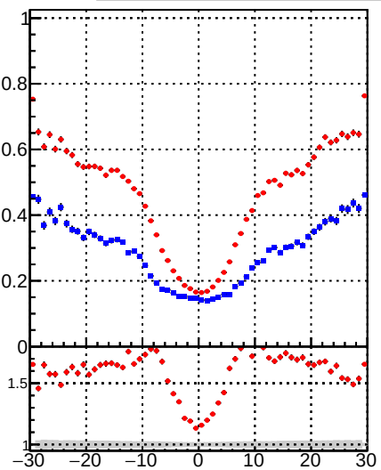
—•— DQM_TT_mkFit_ —•— DQM_TT_mkFit_BDT_
