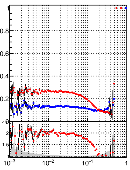
—●— DQM_TT_mkFit —●— DQM_TT_mkFit_BDT
