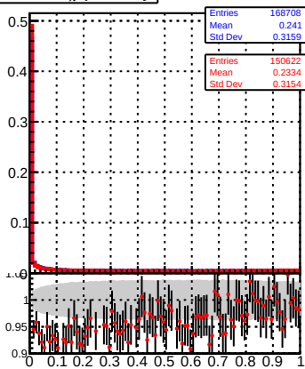
normalized \chi^2 probability
