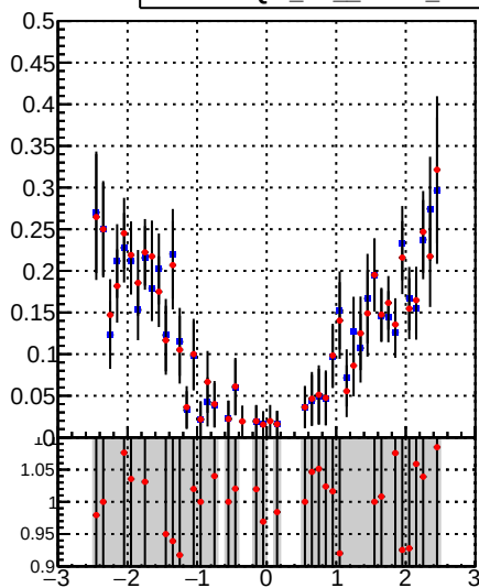
—•— DQM_TT_mkFit_ —•— DQM_TT_mkFit_BDT_
