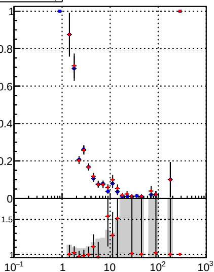
—•— DQM_TT_mkFit_ —•— DQM_TT_mkFit_BDT_
