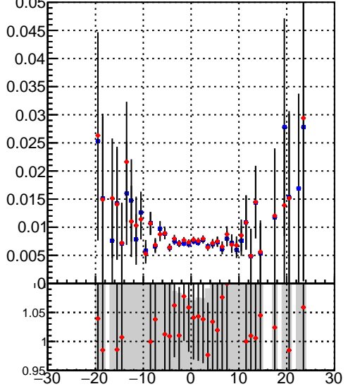
Efficiency vs sim PV z Legend: — DQM_TT_mkFit_ (blue) — DQM_TT_mkFit_BDT_ (red)
