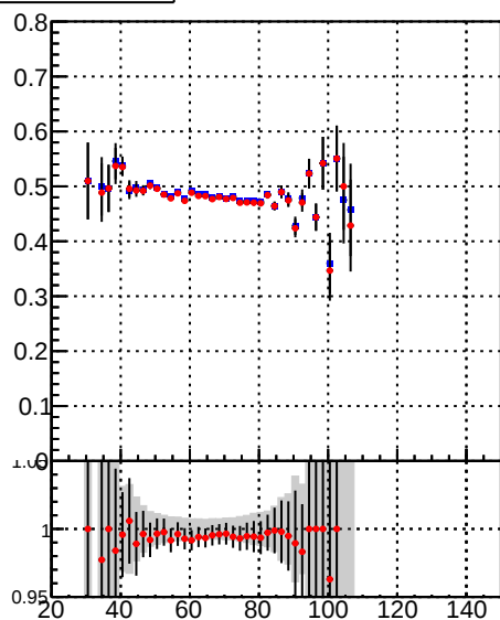
Efficiency vs pu
