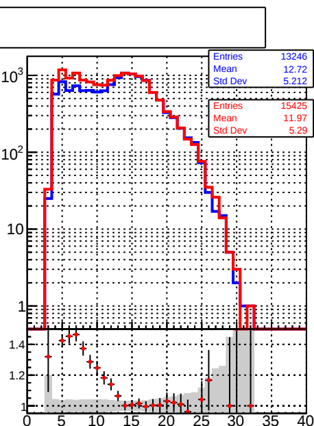
N of reco track vs pT
