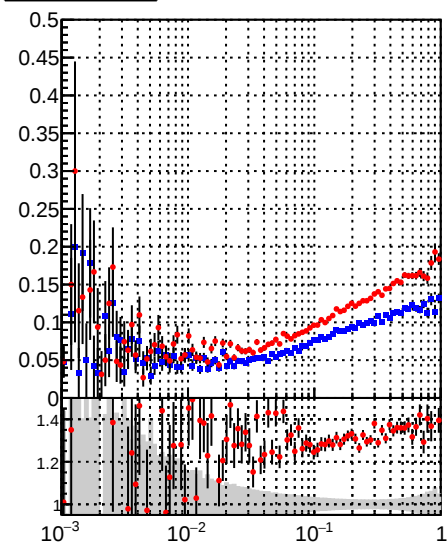
—•— DQM_TT_mkFit_ —•— DQM_TT_mkFit_BDT_
