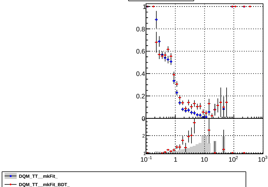
fake+duplicates vs p_T
