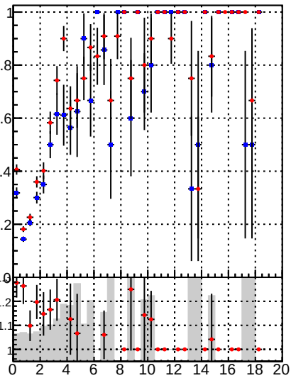
Fake rate vs normalized \chi^2
