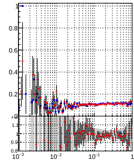
—•— DQM_TT_mkFit_ —•— DQM_TT_mkFit_BDT_
