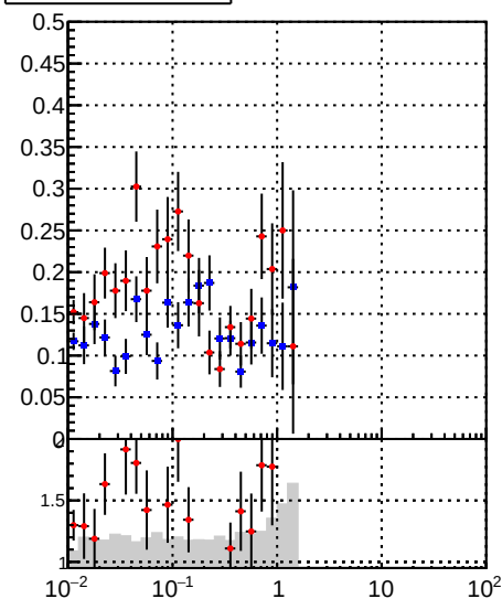
—•— DQM_TT_mkFit_ —•— DQM_TT_mkFit_BDT_
