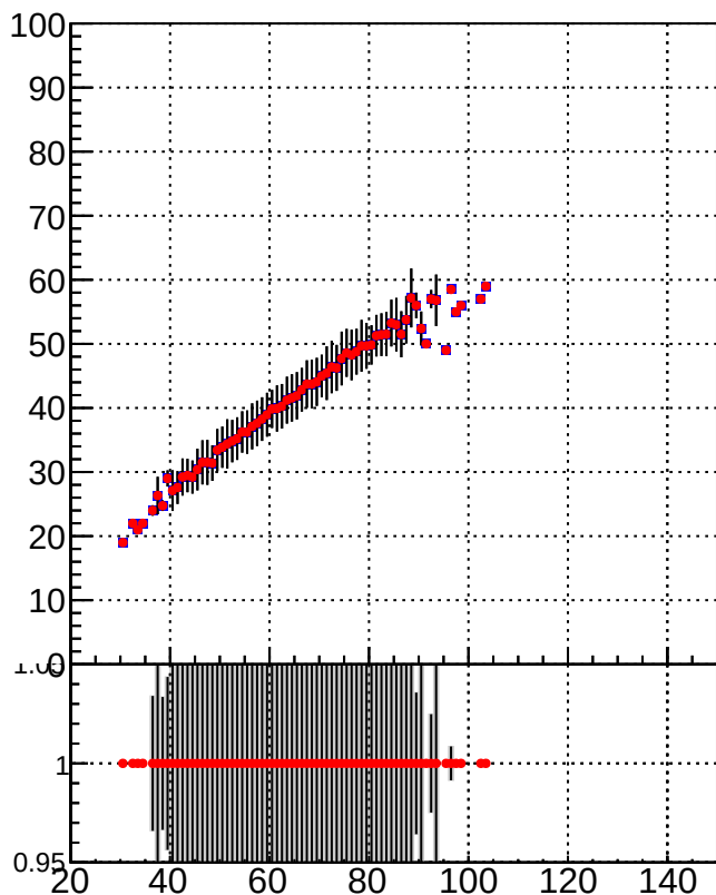
RecoVtx_vs_GenVtx
