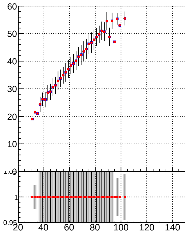
MatchedRecoVtx_vs_GenVtx
