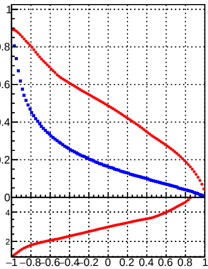
Fake rate vs. MVA1
