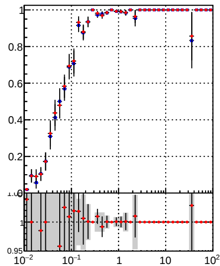
■ DQM_TT_mkFit_ ● DQM_TT_mkFit_BDT_
