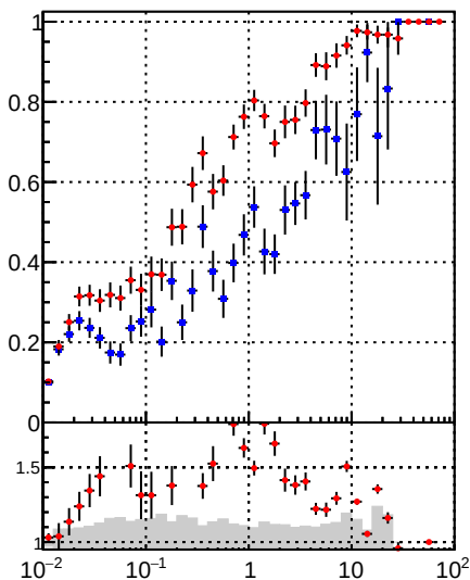
—◆— DQM_TT_mkFit_ —×— DQM_TT_mkFit_BDT_
