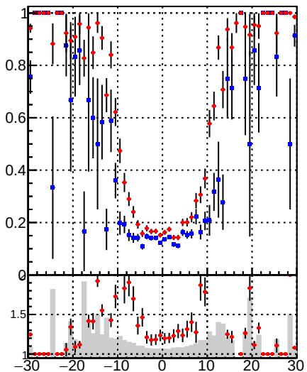
—◆— DQM_TT_mkFit_ —×— DQM_TT_mkFit_BDT_
