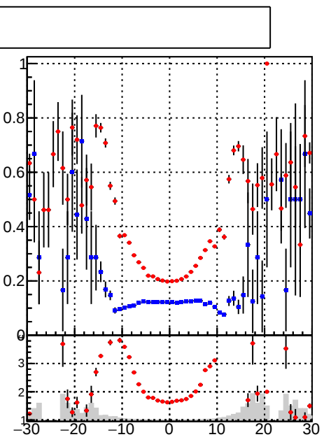
fake+duplicates vs Sim. PV z
