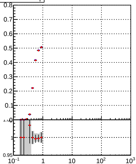
DQM_DisplacedSUSY__mkFit_ DQM_DisplacedSUSY__mkFit_BDT_
