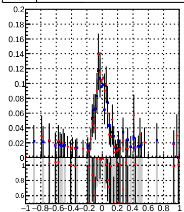
Efficiency vs DQM_DisplacedSUSY_mkFit_BDT_
