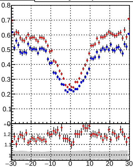
—■— DQM_DisplacedSUSY_mkFit_ —■— DQM_DisplacedSUSY_mkFit_BDT_
