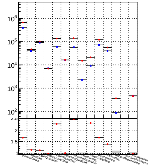
Number DQM_DisplacedSUSY_mkFit_BDT_ 0 0.9876 1 0.9876 2 0.9876 3 0.9876 4 0.9876 5 0.9876 6 0.9876 7 0.9876 8 0.9876 9 0.9876 10 0.9876 11 0.9876 12 0.9876 13 0.9876 14 0.9876 15 0.9876 16 0.9876 17 0.9876 18 0.9876 19 0.9876 20 0.9876 21 0.9876 22 0.9876 23 0.9876 24 0.9876 25 0.9876 26 0.9876 27 0.9876 28 0.9876 29 0.9876 30 0.9876 31 0.9876 32 0.9876 33 0.9876 34 0.9876 35 0.9876 36 0.9876 37 0.9876 38 0.9876 39 0.9876 40 0.9876 41 0.9876 42 0.9876 43 0.9876 44 0.9876 45 0.9876 46 0.9876 47 0.9876 48 0.9876 49 0.9876 50 0.9876 51 0.9876 52 0.9876 53 0.9876 54 0.9876 55 0.9876 56 0.9876 57 0.9876 58 0.9876 59 0.9876 60 0.9876 61 0.9876 62 0.9876 63 0.9876 64 0.9876 65 0.9876 66 0.9876 67 0.9876 68 0.9876 69 0.9876 70 0.9876 71 0.9876 72 0.9876 73 0.9876 74 0.9876 75 0.9876 76 0.9876 77 0.9876 78 0.9876 79 0.9876 80 0.9876 81 0.9876 82 0.9876 83 0.9876 84 0.9876 85 0.9876 86 0.9876 87 0.9876 88 0.9876 89 0.9876 90 0.9876 91 0.9876 92 0.9876 93 0.9876 94 0.9876 95 0.9876 96 0.9876 97 0.9876 98 0.9876 99 0.9876
