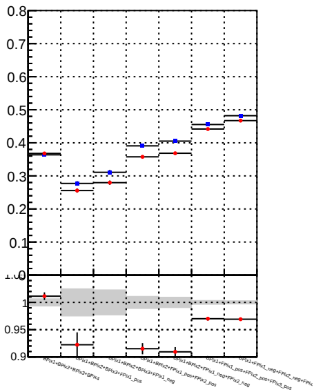
Fake rate vs. DQM_DisplacedSUSY_mkFit DQM_DisplacedSUSY_mkFit_BDT
