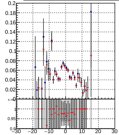
— DQM_DisplacedSUSY_mkFit_ — DQM_DisplacedSUSY_mkFit_BDT_ Efficiency vs. sim PV z
