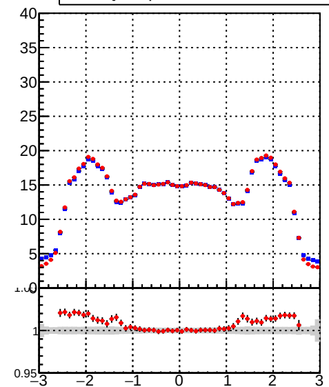
mean hit — DQM_DisplacedSUSY_mkFit_ — DQM_DisplacedSUSY_mkFit_BDT_
