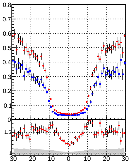
Fake rate vs \Delta d
