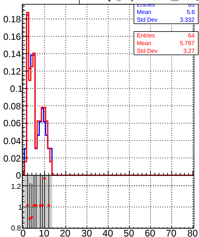
—■— DQM_DisplacedSUSY_mkFit_ —●— DQM_DisplacedSUSY_mkFit_BDT_
