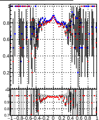
DQM_DisplacedSUSY_mkFit_BDT_
