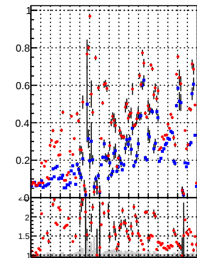
—●— DQM_DisplacedSUSY_mkFit —●— DQM_DisplacedSUSY_mkFit_BDT
