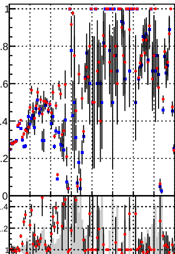
Fake rate vs. —◆— DQM_DisplacedSUSY_mkFit —●— DQM_DisplacedSUSY_mkFit_BDT
