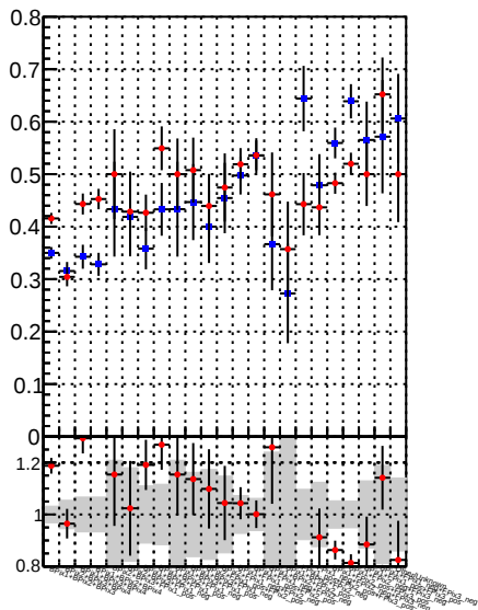
Fake rate vs. — DQM_DisplacedSUSY_mkFit — DQM_DisplacedSUSY_mkFit_BDT
