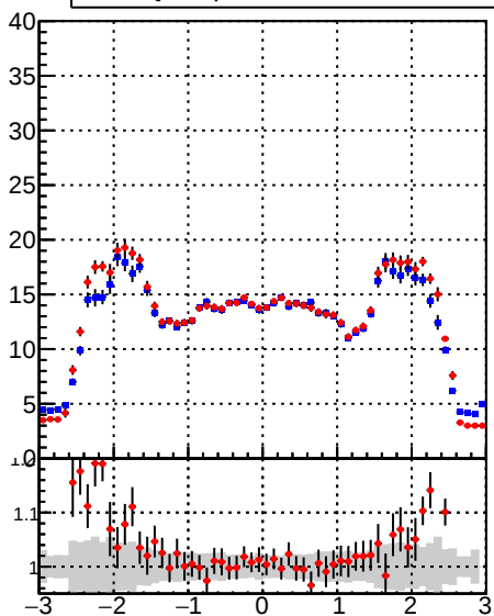
mean hit Legend: — DQM_DisplacedSUSY__mkFit_ — DQM_DisplacedSUSY__mkFit_BDT_
