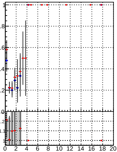
Fake rate vs. \chi^2 for different selection cuts. Legend: \blacksquare DQM_DisplacedSUSY_mkFit, \bullet DQM_DisplacedSUSY_mkFit_BDT.
