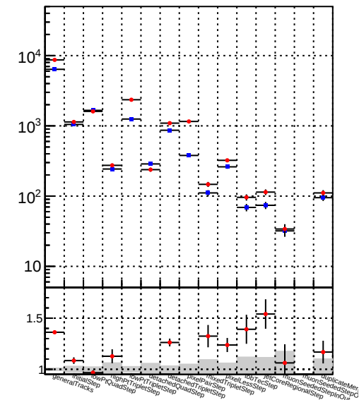
Number DOM DisplacedSUSY mkFit BDT
