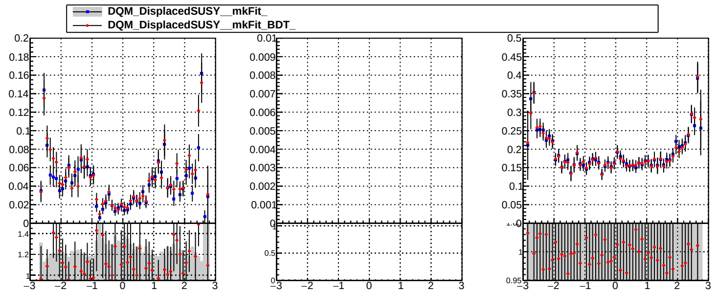
Duplicates Rate vs \phi
