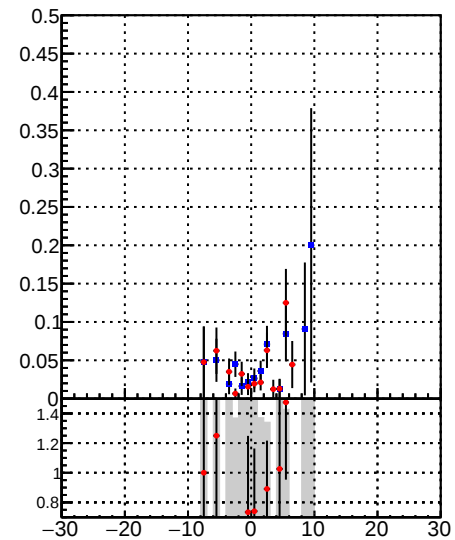
—●— DQM_DisplacedSUSY_mkFit —●— DQM_DisplacedSUSY_mkFit_BDT
