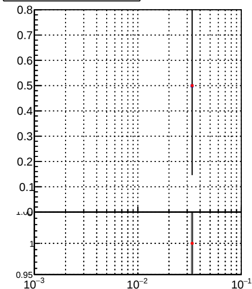
Efficiency vs dr(\text{track}, \text{jet})
