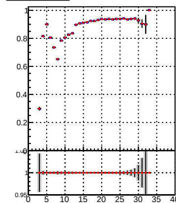
Fake rate vs layer Legend: DQM_DisplacedSUSY_mkFit_ (grey line), DQM_DisplacedSUSY_mkFit_BDT_ (red line)
