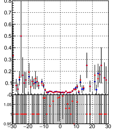
■ DQM_DisplacedSUSY_mkFit_ ● DQM_DisplacedSUSY_mkFit_BDT_ Efficiency
