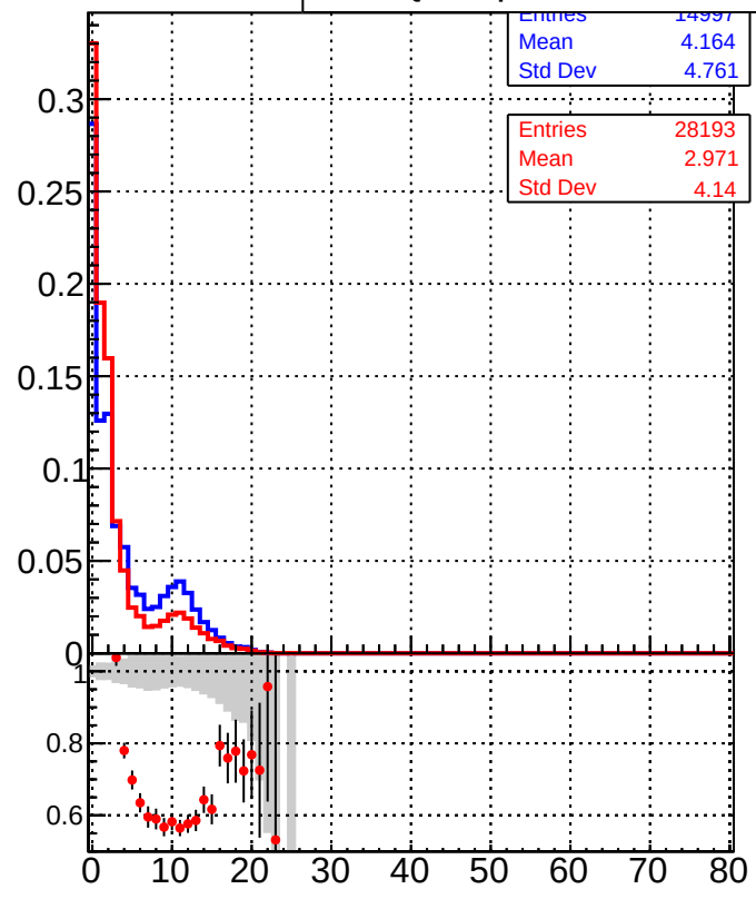
Legend: DQM_DisplacedSUSY_mkFit_ DQM_DisplacedSUSY_mkFit_BDT_
