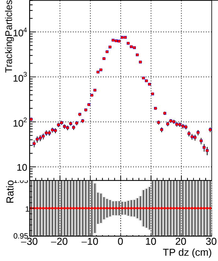
N of simulated track Legend: DQM_DisplacedSUSY_mkFit_ (grey square) DQM_DisplacedSUSY_mkFit_BDT_ (red square)
