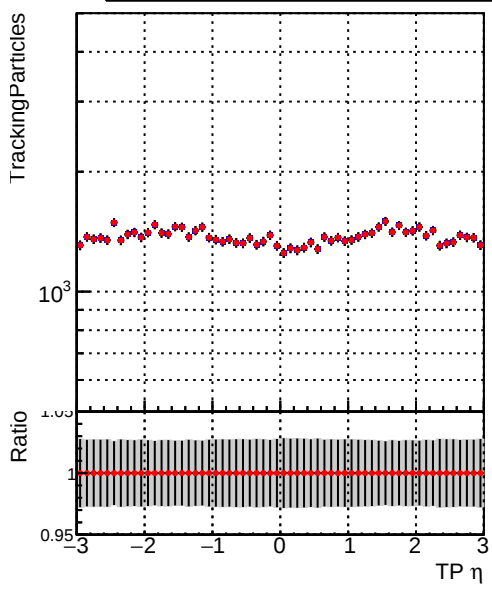
Legend: - \blacksquare DQM_DisplacedSUSY__mkFit_ - \bullet DQM_DisplacedSUSY__mkFit_BDT_
