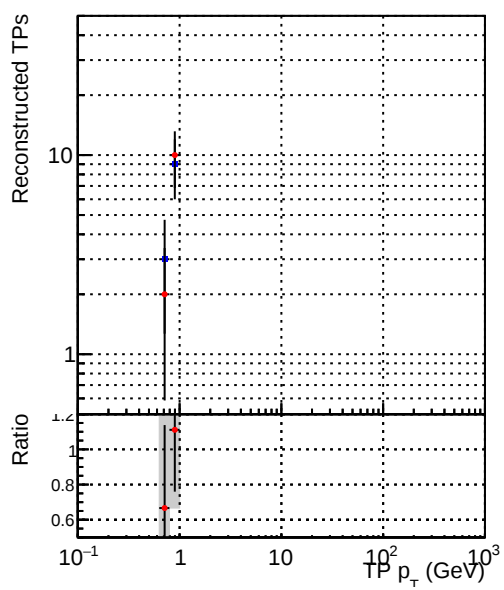
Legend: - \blacksquare DQM_DisplacedSUSY__mkFit_ - \bullet DQM_DisplacedSUSY__mkFit_BDT_
