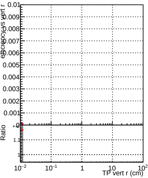
Efficiency vs vertpos Legend: DQM_DisplacedSUSY_mkFit_ (Blue line with dots) DQM_DisplacedSUSY_mkFit_BDT_ (Red line with dots)
