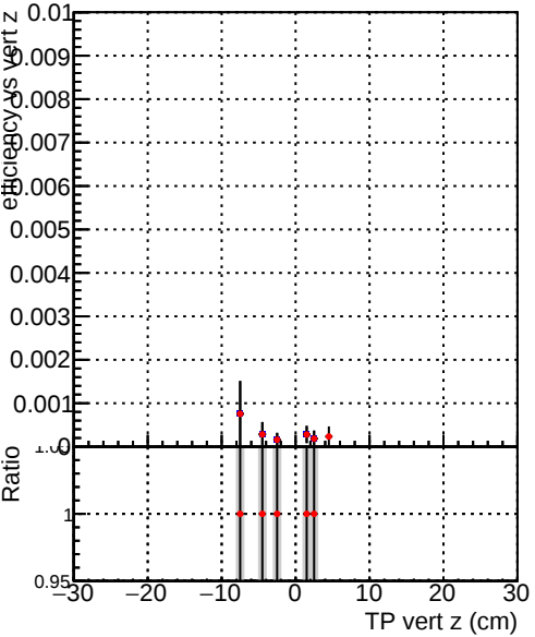
Efficiency vs vertpos Legend: DQM_DisplacedSUSY_mkFit_ (Blue line with dots) DQM_DisplacedSUSY_mkFit_BDT_ (Red line with dots)
