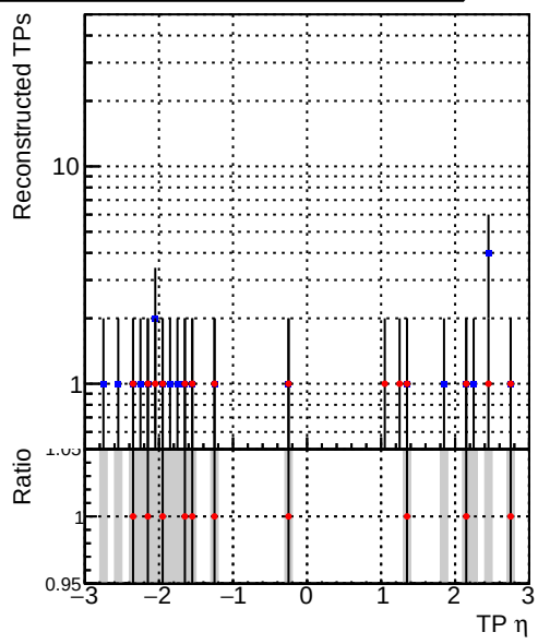
Legend: - Blue dots: DQM_DisplacedSUSY__mkFit_ - Red dots: DQM_DisplacedSUSY__mkFit_BDT_ - Grey shaded band: Ratio uncertainty
