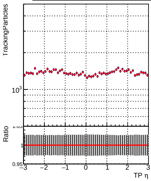
Legend: — DQM_DisplacedSUSY__mkFit_ (blue line) — DQM_DisplacedSUSY__mkFit_BDT_ (red line)
