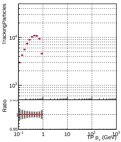
Legend: \blacksquare DQM_DisplacedSUSY__mkFit_ \bullet DQM_DisplacedSUSY__mkFit_BDT_ N of sim
