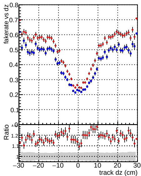
Fake rate vs dz —●— DQM_DisplacedSUSY_mkFit —●— DQM_DisplacedSUSY_mkFit_BDT
