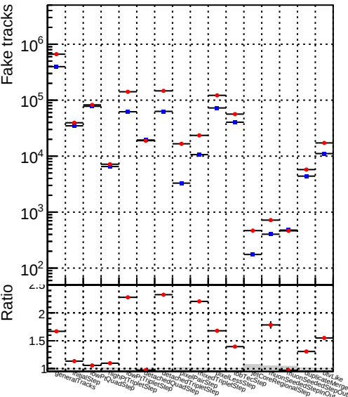
Number —●— DQM_DisplacedSUSY_mkFit_BDT
